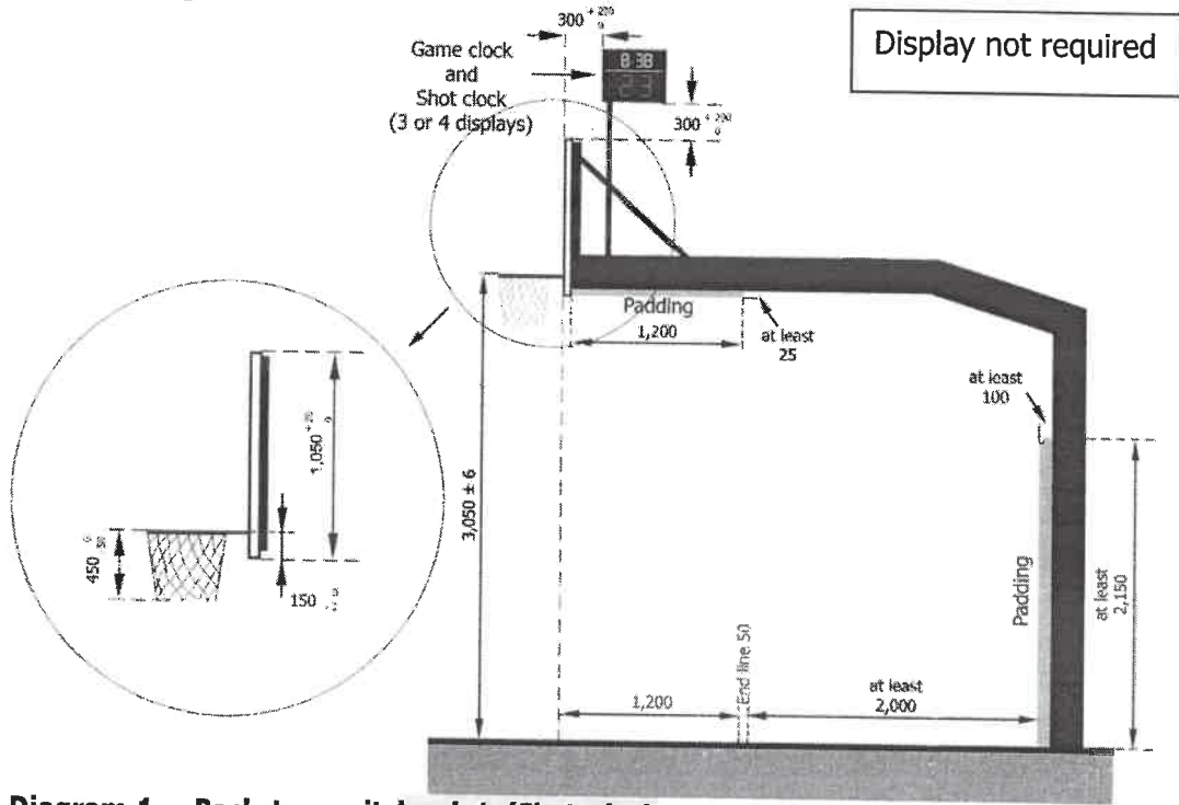
Diagram 1 Backstop unit level 1 (Shot clock option 1)
